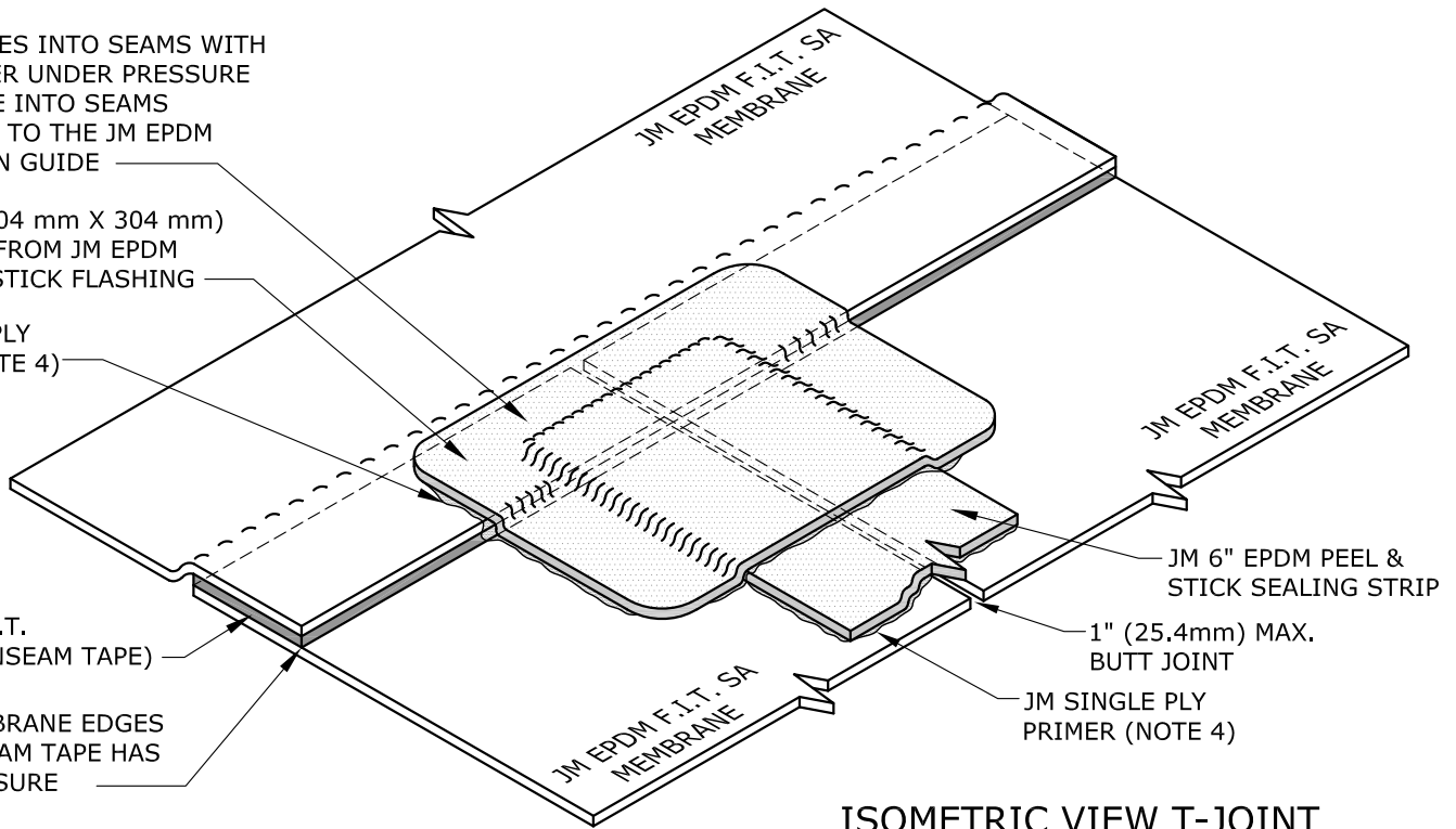
ISOMETRIC VIEW T-JOINT
